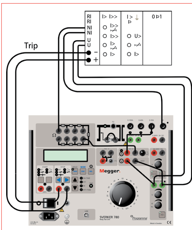
Testing the pick-up and drop-out using SVERKER 780
