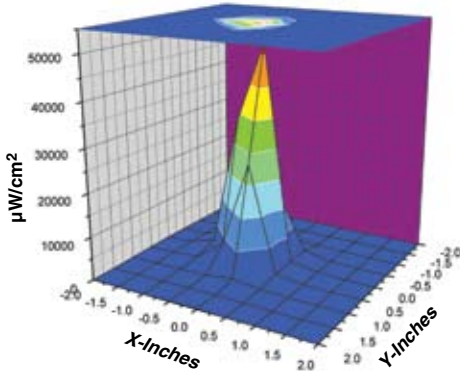
SURFACE CONTOUR PROFILE AT 6 IN (15 CM)
