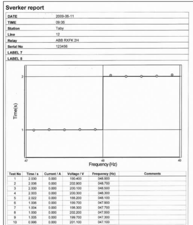
Frequency relay test report
